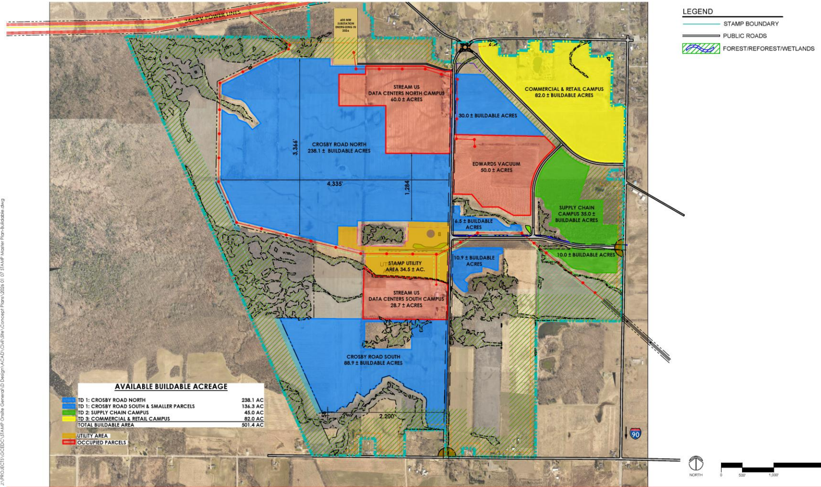
STAMP - MASTER PLAN - BUILDABLE WNY SCIENCE AND TECHNOLOGY ADVANCED MANUFACTURING PARK (STAMP) JANUARY 2026
