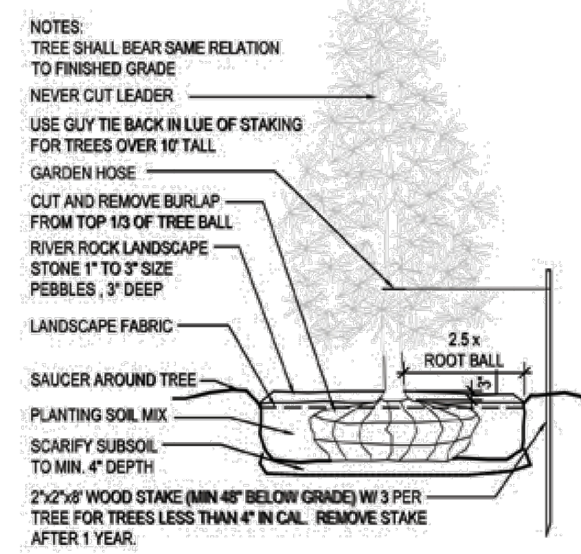
PLANTING DETAILS SCALE: NTS
